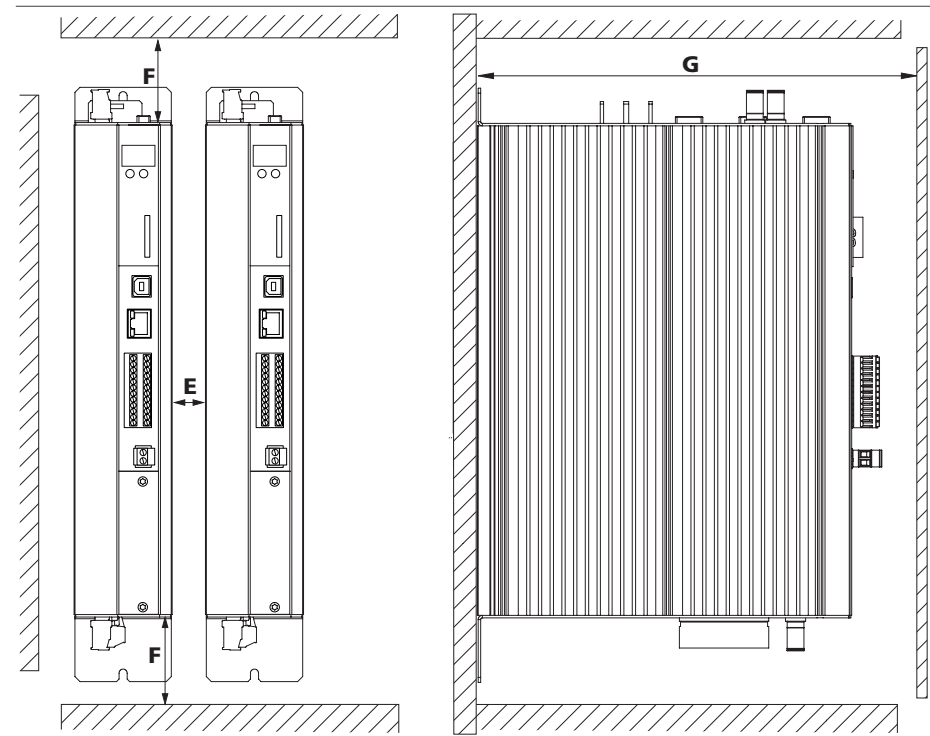
Fig. 2.1 Installation distances in case of air cooling, schematic representation for BG1 to BG6a
