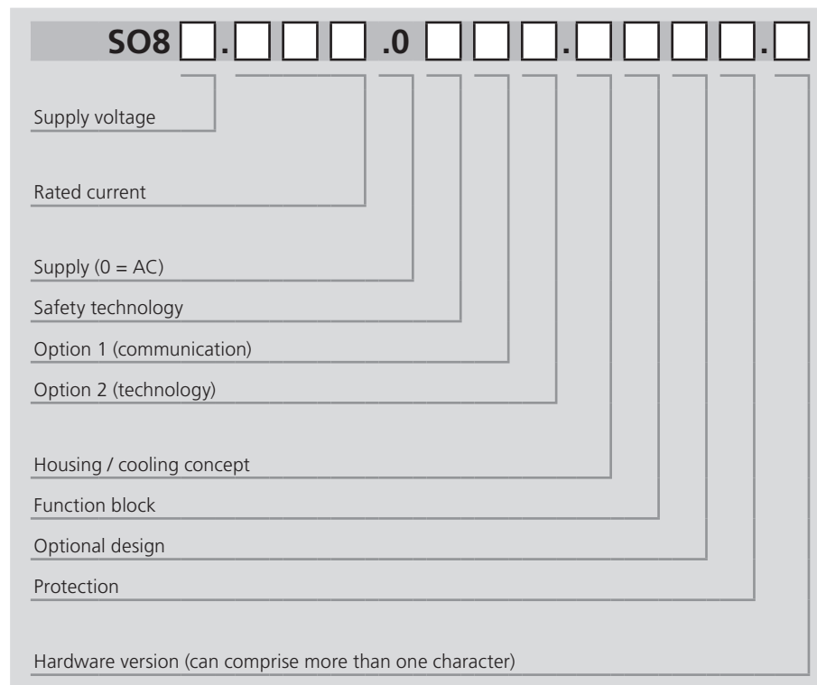
Fig 0.1 Order code ServoOne Single-Axis System
