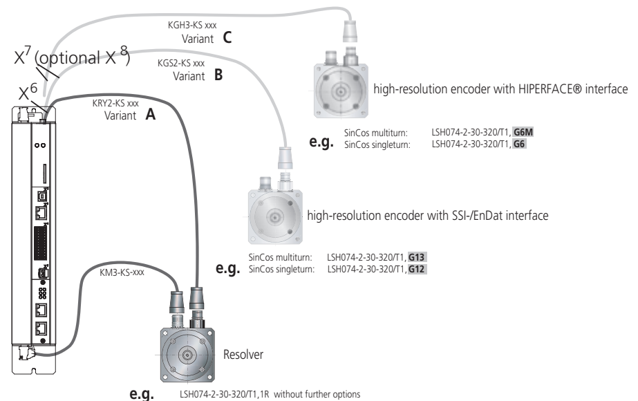
Fig. 3.15 Assignment motor/encoder cable
