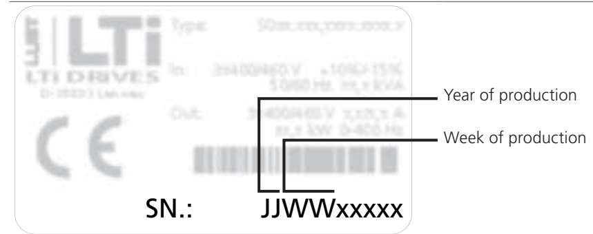
Fig 0.2 Rating plate hardware ServoOne Single-Axis System
